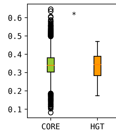
GC3s
