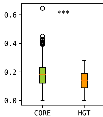
Nc
