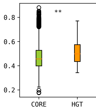
Fop
